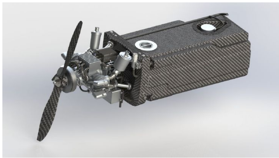
Engine unit
