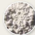
Calcium Carbonate
