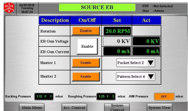
Touch screen HMI based operation
