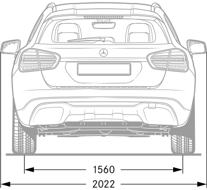
All figures in millimetres. The illustrated dimensions are mean values. They are valid for vehicles in basic specification and in unladen condition.
