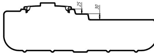
CROSS-SECTION A-A SCALE 1:4
