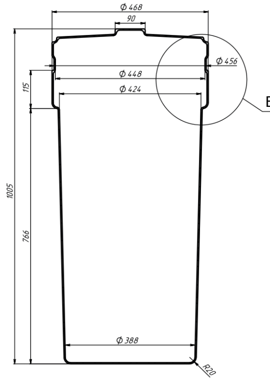
CROSS-SECTION A-A SCALE 1:4
