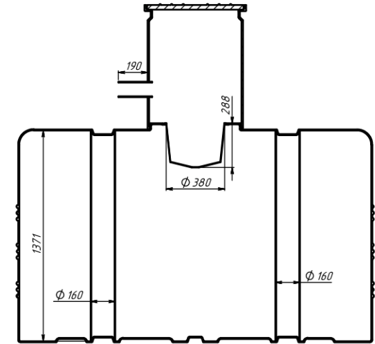
CROSS-SECTION B-B SCALE 1:12
