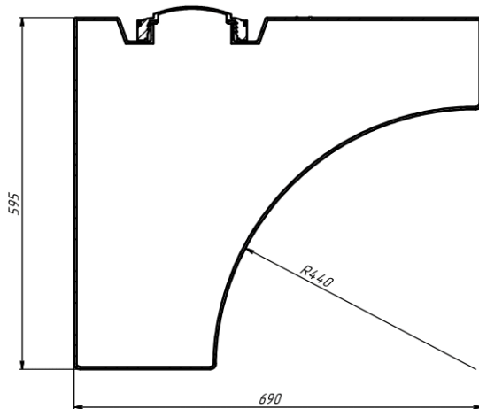
CROSS-SECTION A-A SCALE 1:4
