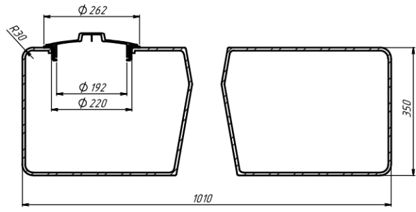
CROSS-SECTION B-B
