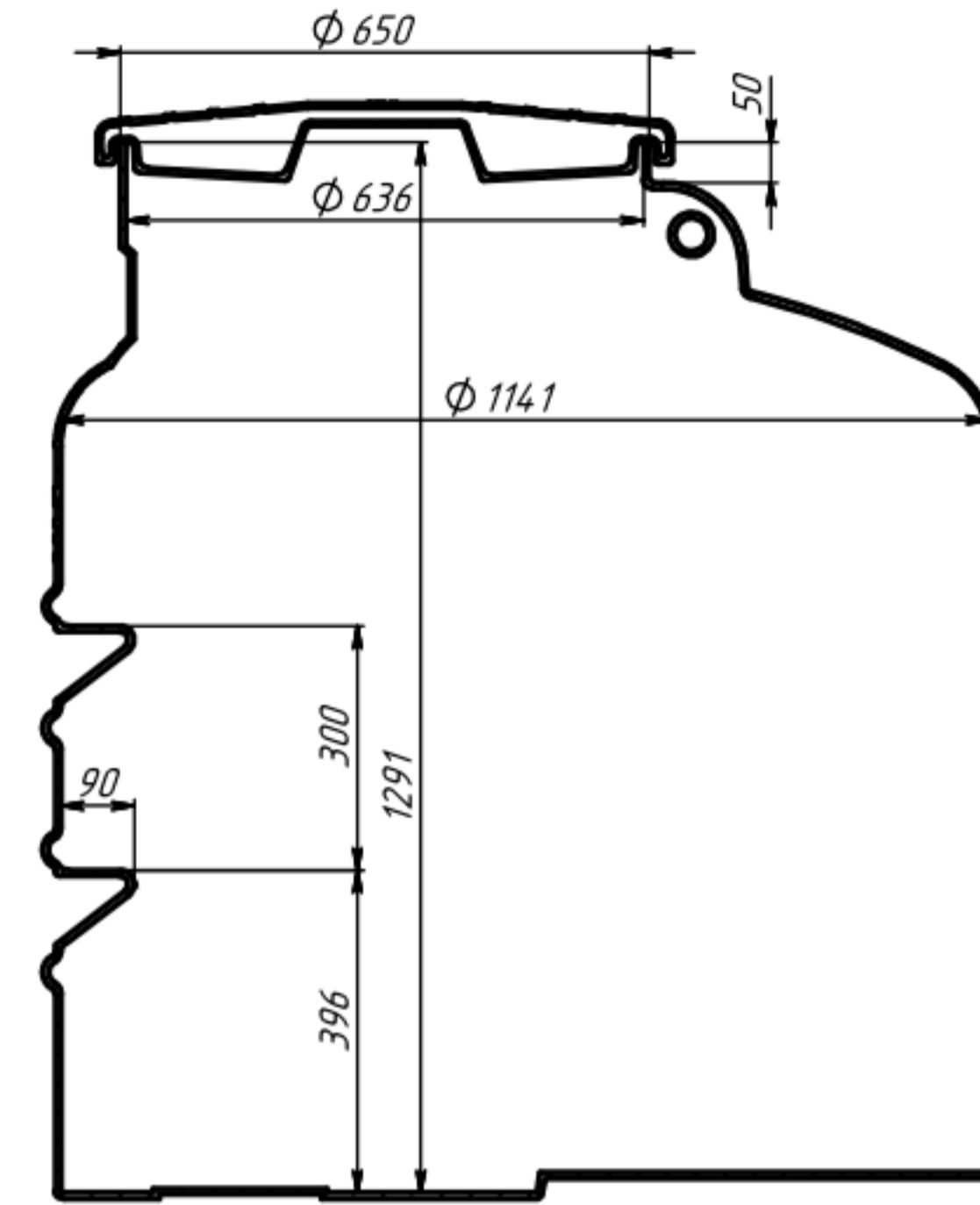
CROSS-SECTION A-A SCALE 1:8
