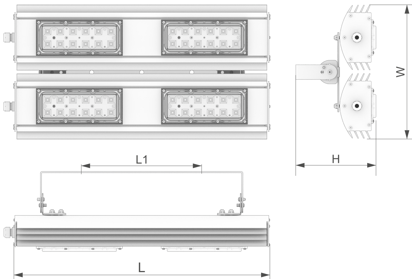
VECTOR STRADA-D-200-ABC-П
