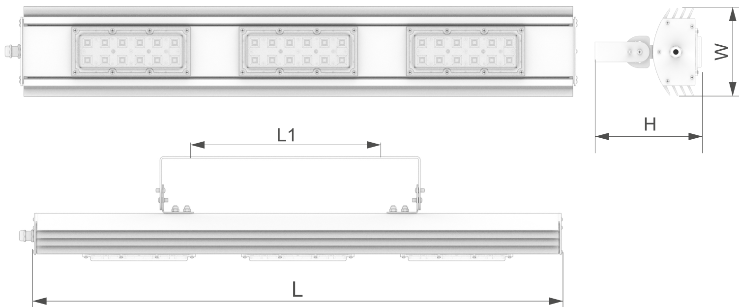
VECTOR STRADA-D-150-ABC-П
