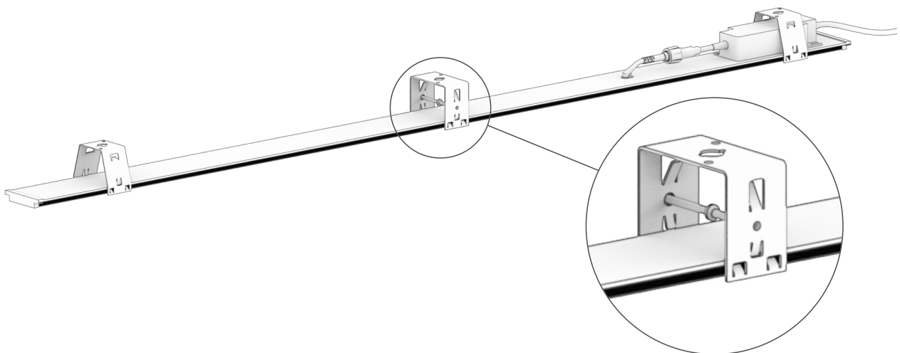
Mounting Brackets - 2 anti-vandal bracket H - 50 mm
