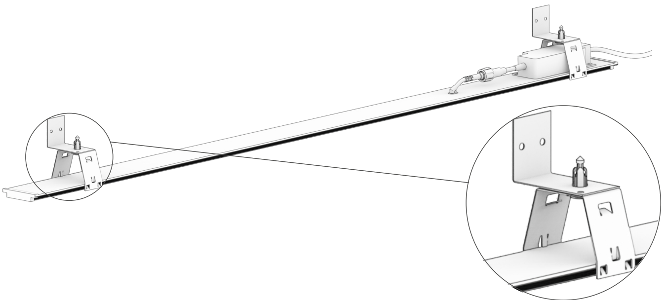
Mounting Brackets - 4 L-shaped (for facades)
