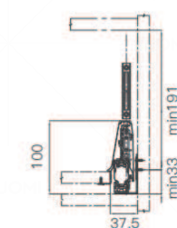
3. 箱体所需空间 Space requirements in cabinet
