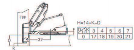
Full Overlay 直臂
