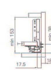
3. 箱体所需空间 Space requirements in cabinet
