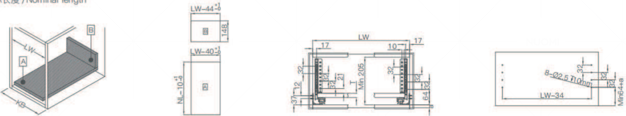
1. 箱体内部所需空间 Space requirements in cabinet
