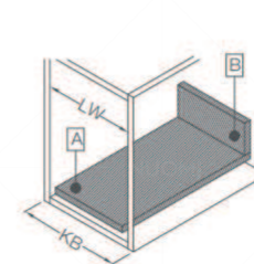
1. 箱体所需空间 Space requirements in cabinet
