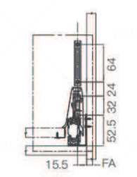
FA 面板重叠部分 Front board overlap
