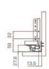
FA 面板重叠部分 Front board overlap
