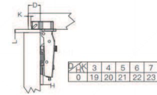
Full Overlay 直臂
