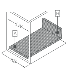
1. 箱体所需空间 Space requirements in cabinet
