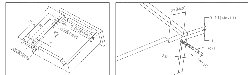
抽屉尺寸 Drawer size
