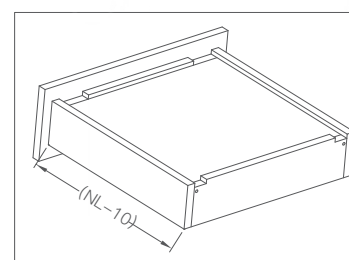
抽屉尺寸和钻孔(mm) Drawer size and drilling
