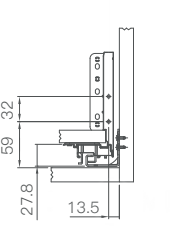
FA 面板重叠部分 Front board overlap
