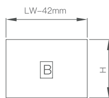
LW 柜体净宽 / Inner cabinet width 背板减尺: 42mm
