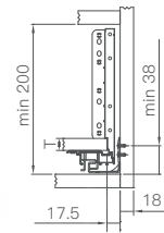
3. 箱体所需空间 Space requirements in cabinet
