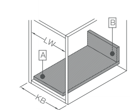
1. 箱体所需空间 Space requirements in cabinet
