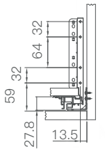
FA 面板重叠部分 Front board overlap
