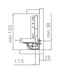
3. 箱体所需空间 Space requirements in cabinet
