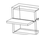
层板 (含灯具) 安装在柜子里 Install the shelf (with light bar) to the cabinet
