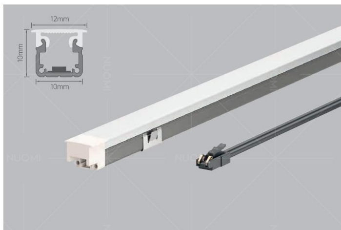
嵌入式灯条 (灯罩翻边) -DIY 配件 BUILT-IN LIGHT BAR (FLANGED LAMP SHADE) - DIY ACC.
