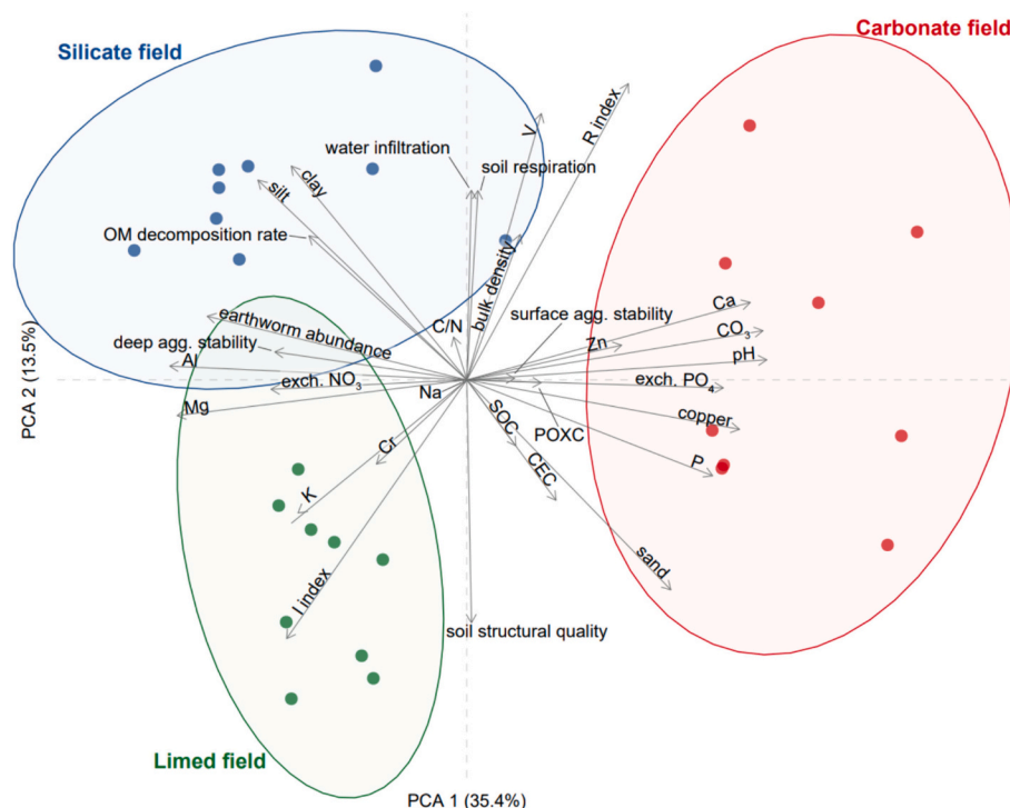
Fig. 3. Biplot showing the results of a principal component analysis (PCA) of soil fertility parameters. The input data is the complete dataset for all treatments. The first two principal components (PCA 1 and PCA 2) are the two dashed axes. The share of explained variance by each PCA is given in brackets. Each arrow represents a loading vector, indicating the magnitude and direction of a fertility parameter's contribution to the component. Each dot represents a plot from the Carbonate field (blue), Silicate field (red) or Limed field (green). Each ellipse encloses the region that contains plots from each field, with a 95 % confidence level.
