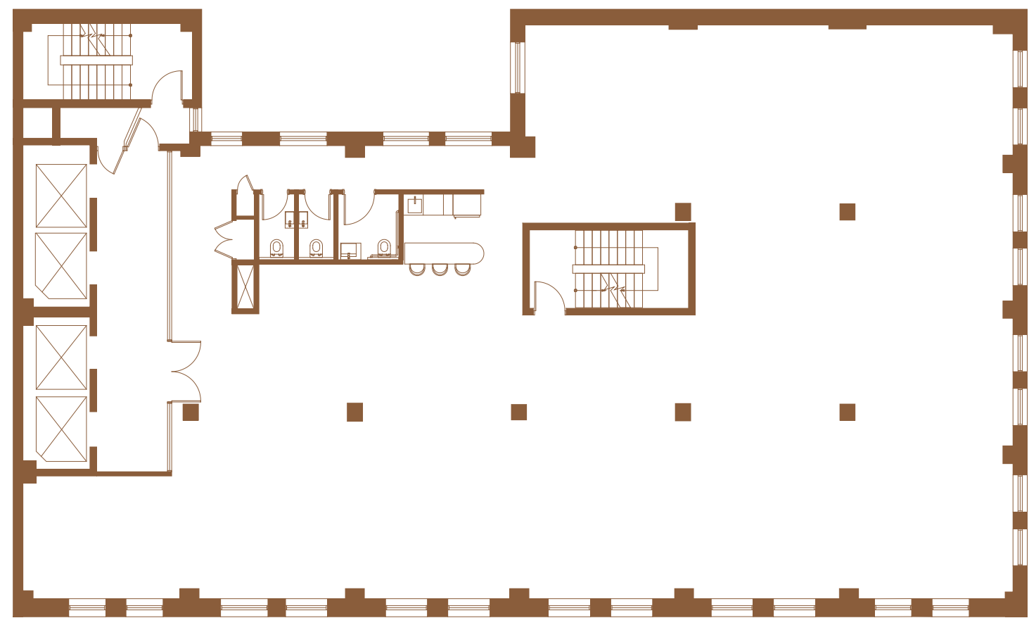
12TH FLOOR | OPEN
